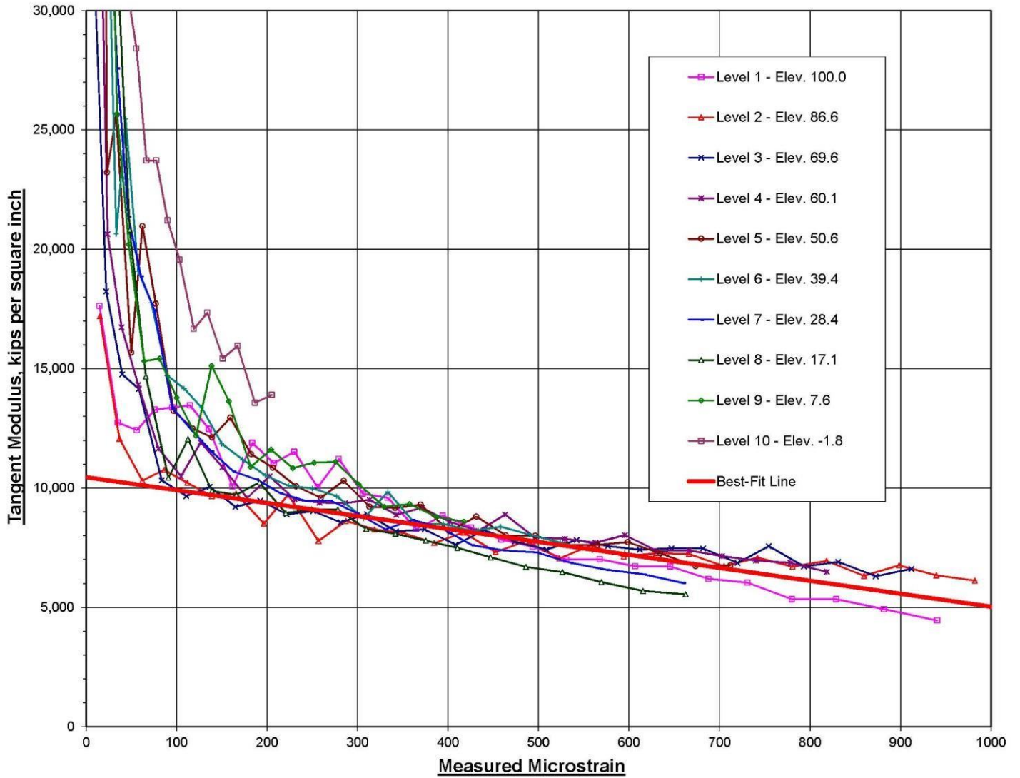
Figure 1. Tangent Modulus Versus Measured Microstrain from an Instrumented Static Load Test.
