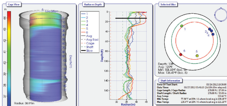
Figure 1: TIP Reporter screen shot. On the left is a 3D image of the effective shape of the shaft that can be rotated to any orientation. The center image plots effective radius versus depth. On the right, a "horizontal slice" shows the inner cage radius (inner circle), the nominal shaft diameter (middle circle), and outer shaft profile (outer circle). The slice is from the upper, temporary cased portion of the shaft; its location is indicated in the center image by a horizontal line.
