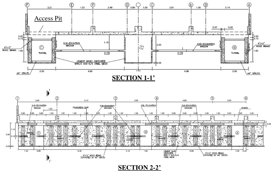
Fig. 2 Top: Maneuver Tunnels and sub-excavation windows, Bottom: Retaining system and details
