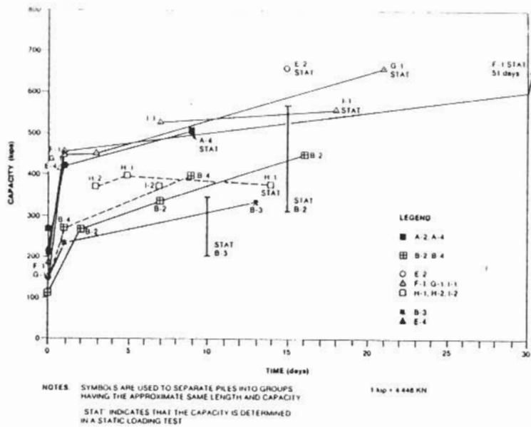
FIG. 9. Capacity versus Time
