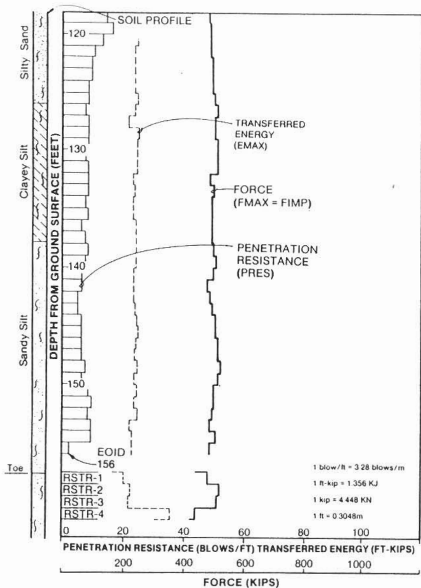
FIG. 3. Driving Diagram for Pile B-2
