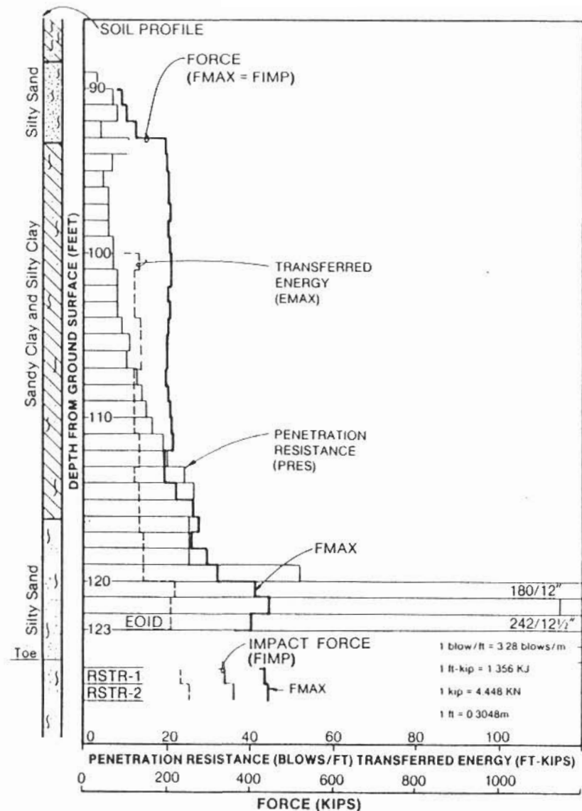
FIG. 2. Driving Diagram for Pile A-1
