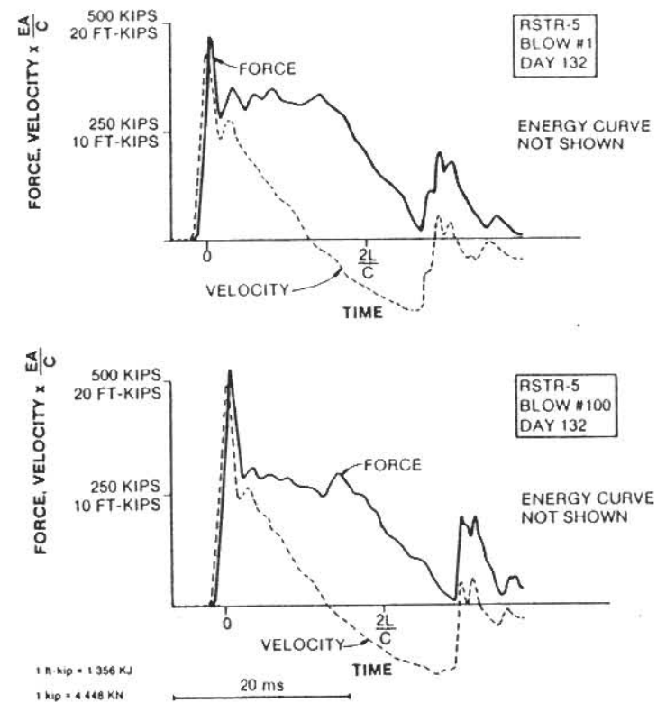
FIG. 6. Pile B-2 Force, Velocity, and Energy Wave Traces (RSTR-5)
