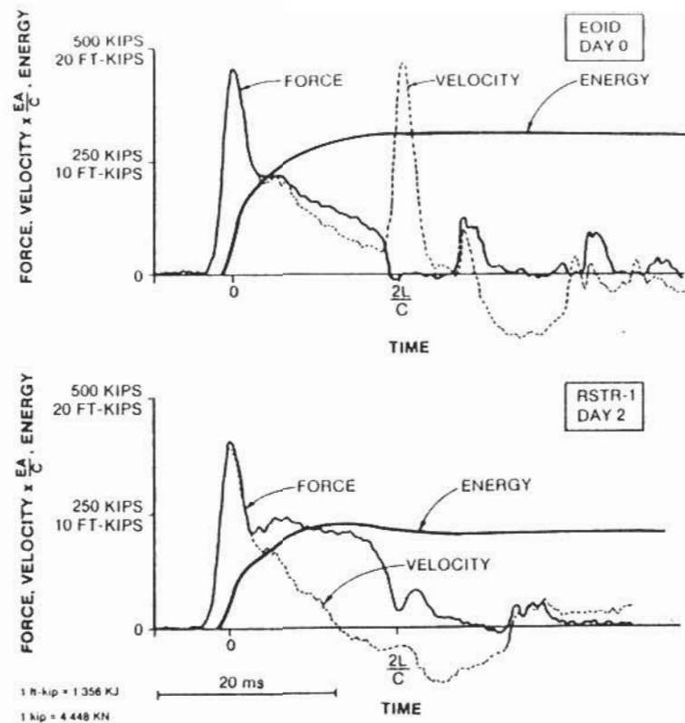
FIG. 4. Pile B-2 Force, Velocity, and Energy Wave Traces (EOID and RSTR-1)
