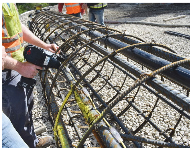
Figure 13. TIP wire attachment to a drilled shaft cage.
