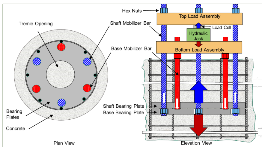
Figure 38. General schematic of a Top-Loaded Bi-Directional Test.
