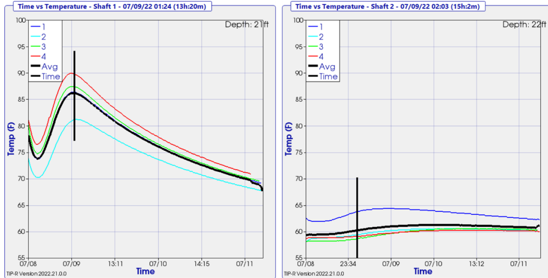
Figure 17. TIP Results: Temperature vs Time Comparison of Lowest Node in Two Project Shafts
