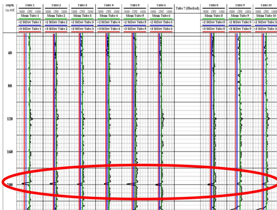
Figure 24. GGL results on a density vs depth plot.
