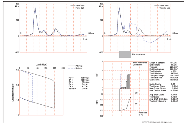
CAPWAP Data Output Graphs
