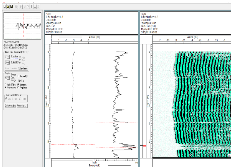
Figure 19. Analysis software showing first arrival time (FAT), energy, and waterfall diagram (right).
