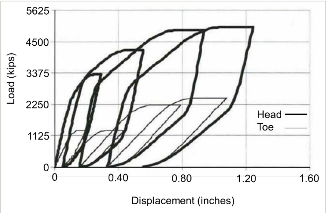
Figure 7. Dynamic load test load-movement envelope.
