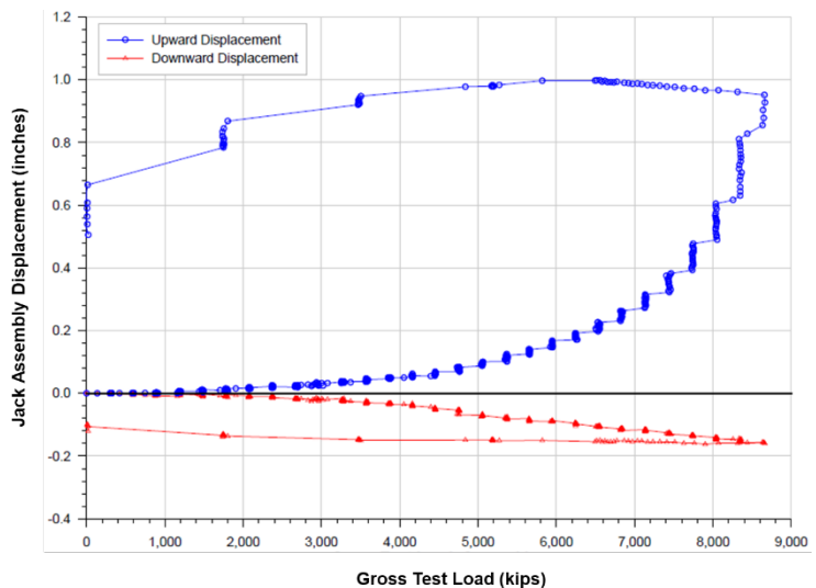
Figure 35. Upper and lower bearing plate displacements.
