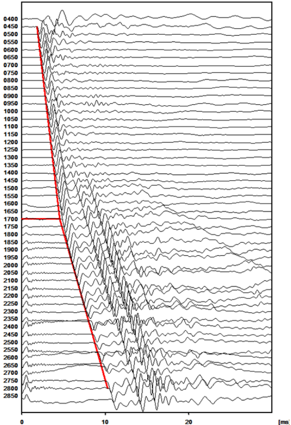
Figure 52. Parallel seismic test results.
