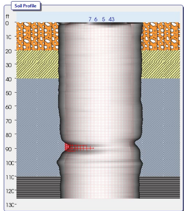
Figure 16. TIP Results: 3D shaft interpretation.
