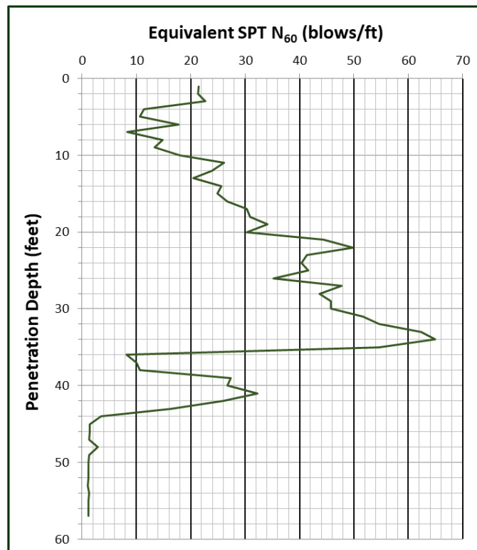
Figure 48. Equivalent SPT N_{60} values versus depth.
